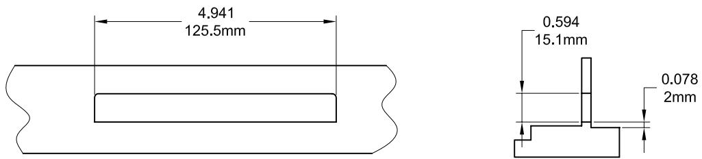
Profile Cut Out
